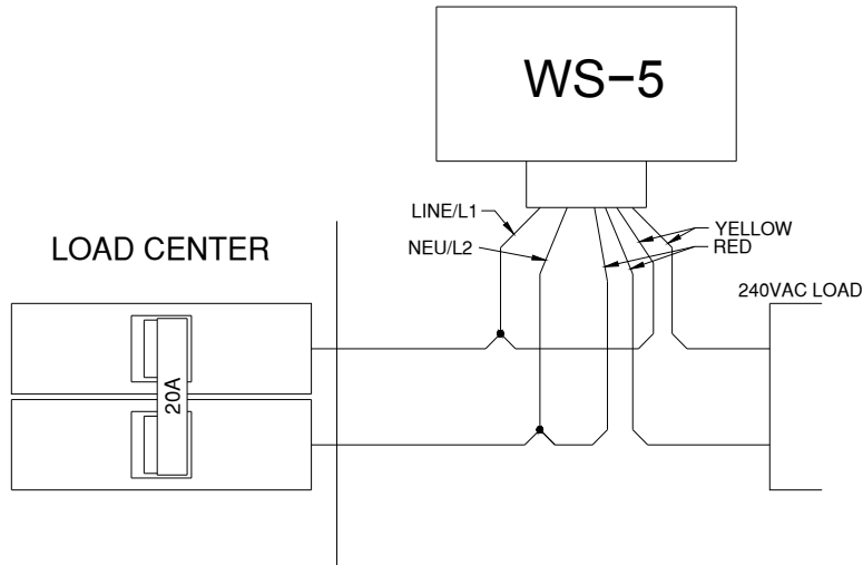
240VAC In, 240VAC Load, Heat Cable or Similar (Strap WS-5 for 240VAC Power)
