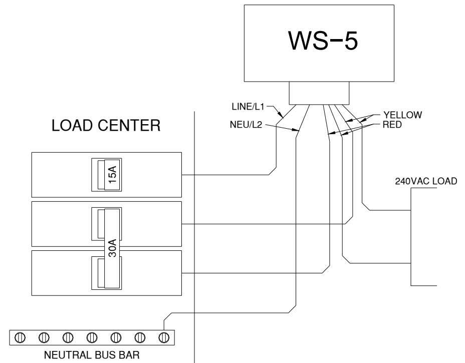
120VAC In, 240VAC Load, Heat Cable or Similar (Strap WS-5 for 120VAC Power)
