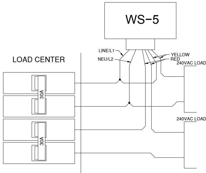
240VAC In, Dual 240VAC Loads (Strap WS-5 for 240VAC Power)
